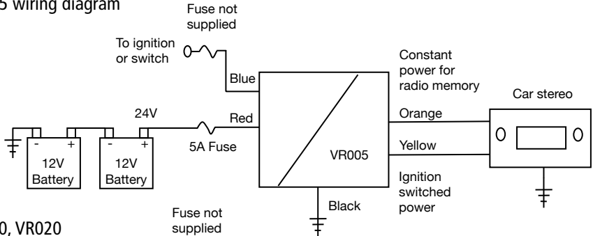
VR010, VR020 & VR030 wiring diagram
